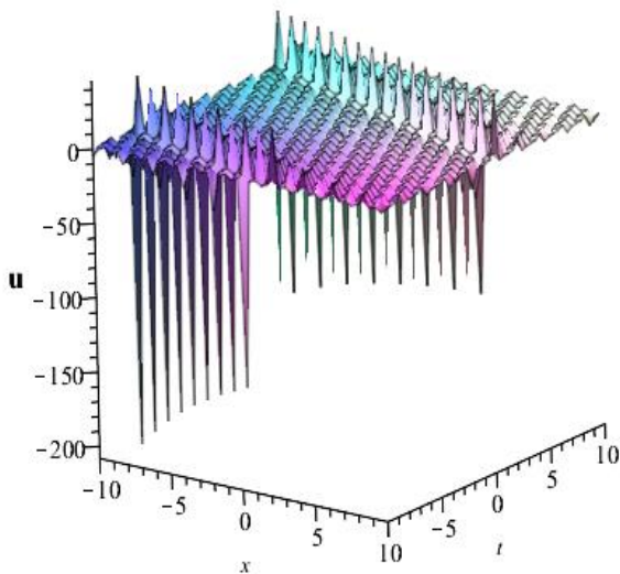
Fig-3.4: Doubly-periodic wave solution for a_0 = 1, k_1 = 1, k_2 = 2.5 of u_{15} .
