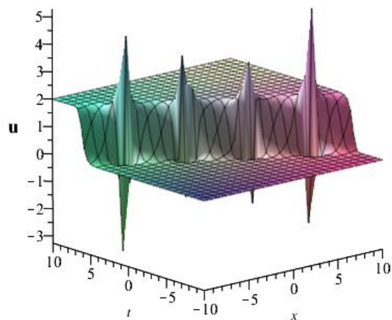
Fig-3.5: Kinky periodic lump wave solution for a_0 = 1, k_1 = 1, k_2 = 2 of u_{19} .
