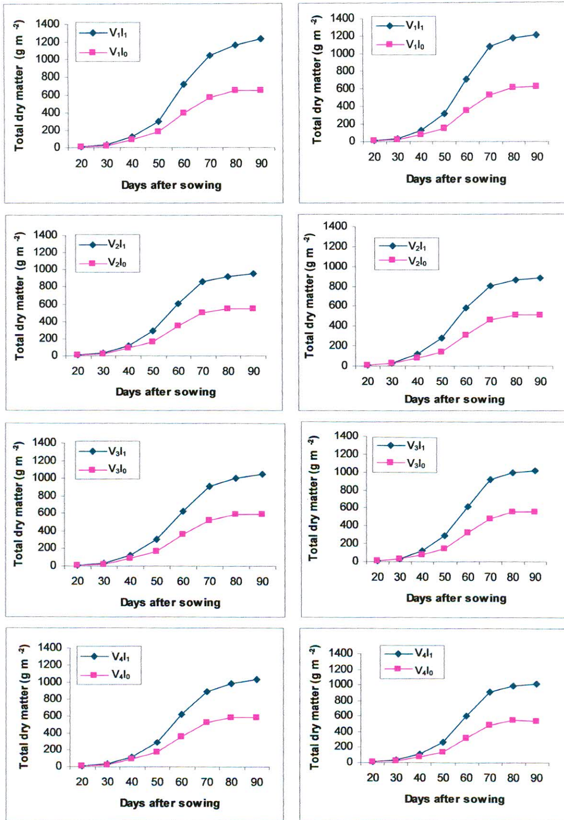
Figure 1b: Effects of soil moisture on total dry matter (TDM) of four wheat varieties at different growth stages in 2005-06 experiment (left) and in 2006-07 experiment (right).
