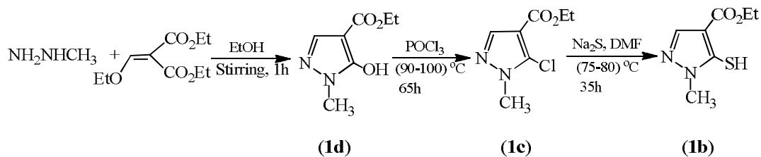
Scheme 1.1
