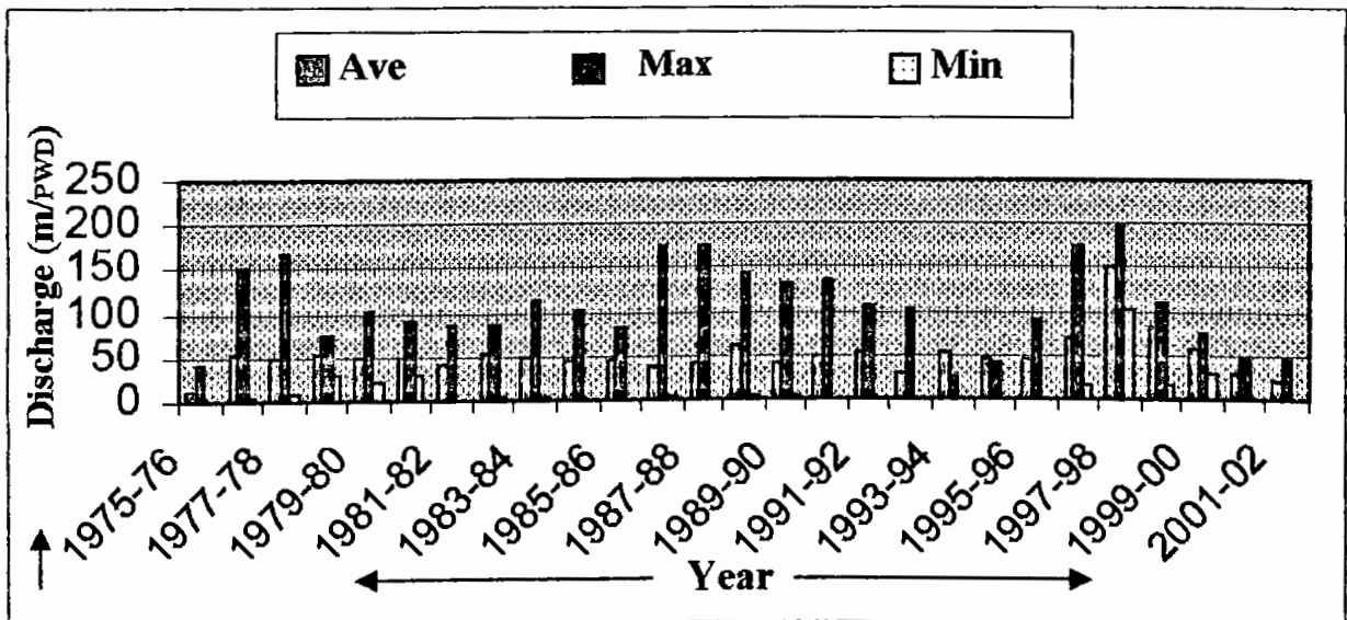
Figure-3.10: Annual discharge at Nawhata station from 1975-76 to 2001-02 (station No.-261).
