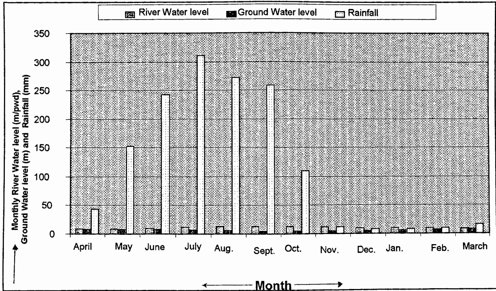
Fig:-3.7: Monthly water level of Sibiu-Baranai river, elevation of ground water table at well No.-38 and rainfall at Tanore station of the last 21 years.
