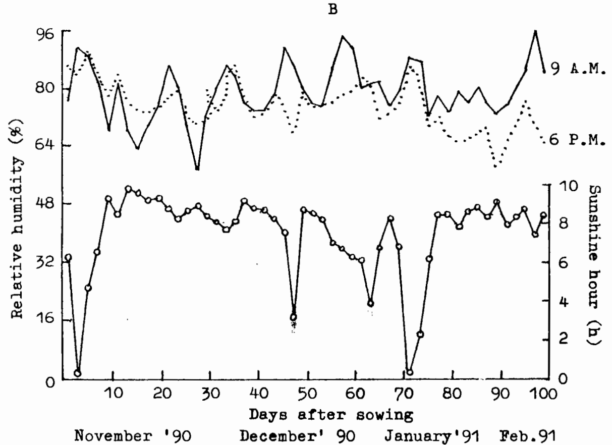
Figure. 0.3. Meteorological information during the crop period. A. Max=maximum, Min=minimum and S=soil temperature(°C) and total rainfall(histogram). B. Relative humidity at 9 A.M.(continuous line), 6 P.M.(dotted line) and sunshine hour (O-O).
