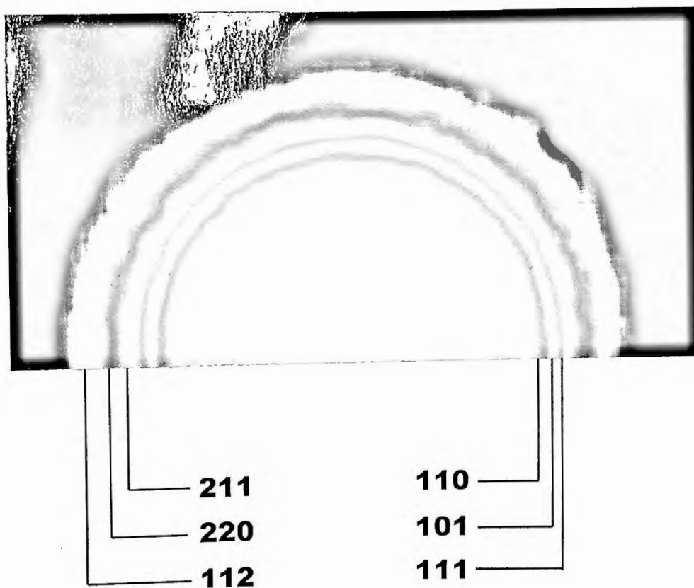
Figure 4.8(b): Electron Diffraction pattern of MnO 2 film of thickness 380nm deposited at a substrate temperature 593K.
