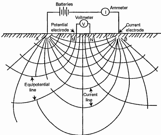
Fig.-4.1b: Electrical circuit for resistivity determination and electrical field for a homogeneous subsurface stratum
